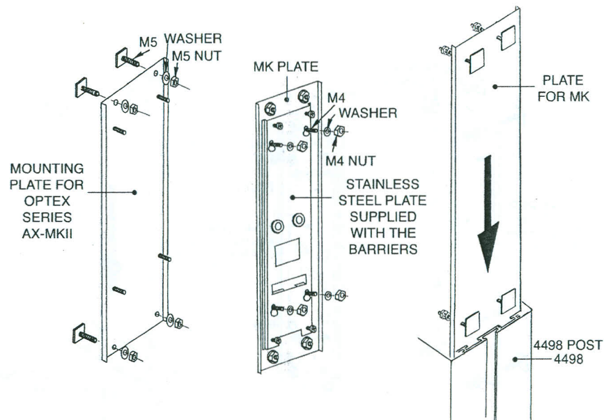
Mounting fastening of the MK plate
